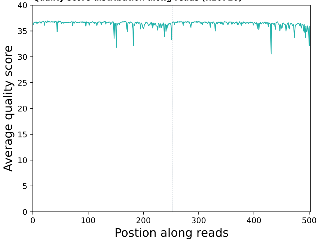
Quality score distribution along reads (R10716)
